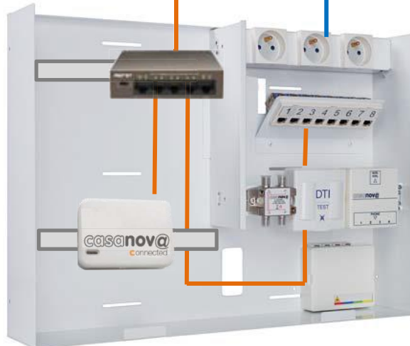
Switch PoE
