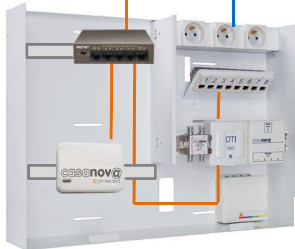
Switch PoE
